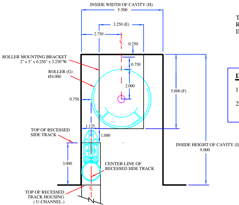
PLACEMENT OF 4" ROLLER, 5" ROLLER MOUNTING BRACKET AND RECESSED SIDE TRACK (V3)
