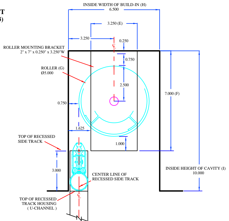
PLACEMENT OF 5" ROLLER, 7" ROLLER MOUNTING BRACKET AND RECESSED SIDE TRACK (V3)
